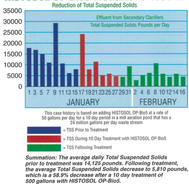
This graph depicts biological enhancement and improved polymer bio-production resulting in over-all reduction in effluent total suspended solids.
