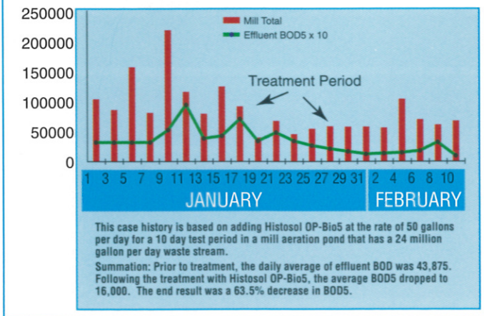
This graph depicts biological enhancement resulting in over-all reduction in final effluent BOD.
