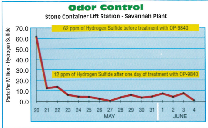
This graph depicts H 2 S reduction with 80.6% reduction within the first 24 hours of treatment.
