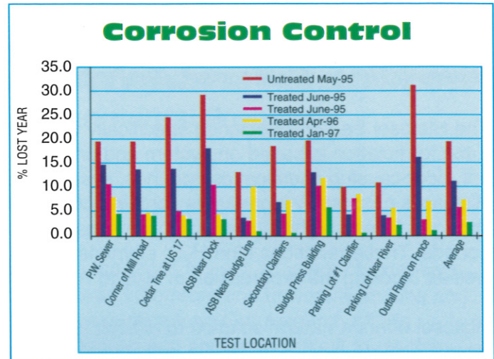
This graph depicts an 87.5% reduction in corrosion over a three-year period. Substantiated by copper corrosion coupon testing.
